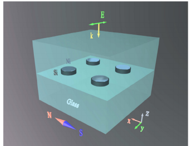
Fig. 1. Scheme of the model. 5-nm-thick nickel film covers 220-nm-thick silicon nanodisks. Subdiffractive array is organized by nanodisks with interparticle distance of 200 nm forming the magnetophotonic metasurface. The metasurface is embedded in a dielectric environment with n = 1.5 . An external magnetic field is applied along the X direction, polarization of light is oriented along Y axis and the wavevector is collinear with Z axis.
