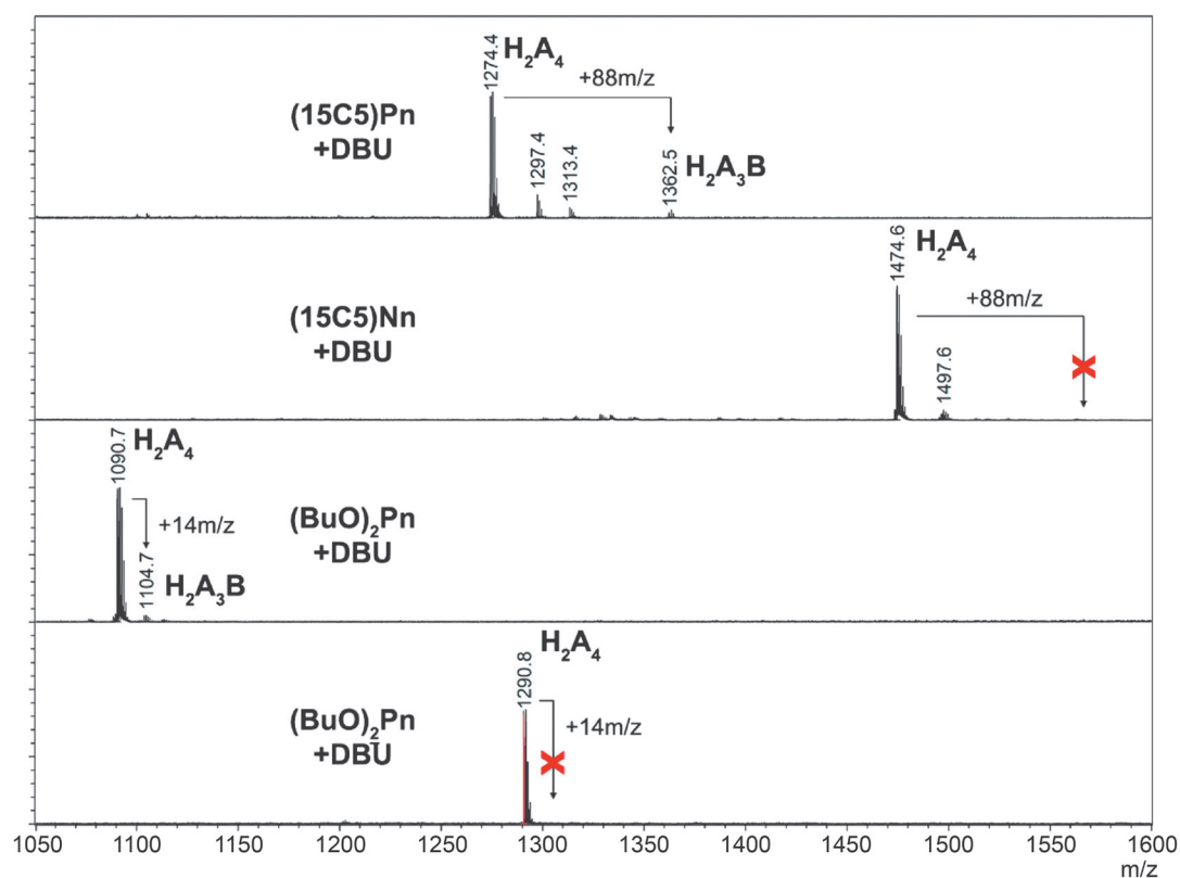
Figure 2. MALDI-TOF mass-spectra of reaction mixtures, formed upon cyclotetramerization of dinitriles in the presence of DBU in refluxing n -pentanol. “A” stands for intact isoindoline unit as a part of (na)phthalocyanine, “B” stands for the unit formed because of nucleophilic substitution.
