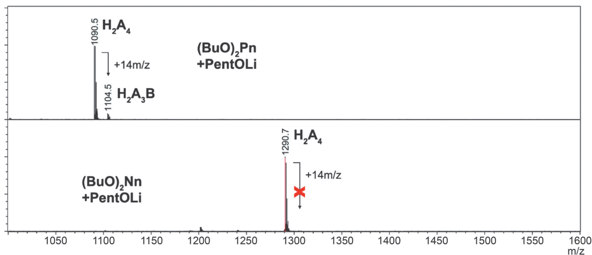
Figure 4. MALDI-TOF mass-spectra of reaction mixtures, formed upon cyclotetramerization of butoxy-substituted dinitriles in the presence of PentOLi in refluxing n -pentanol. “A” stands for intact isoindoline unit as a part of (na)phthalocyanine, “B” stands for the unit formed because of nucleophilic substitution of BuO- with PentO-groups.
