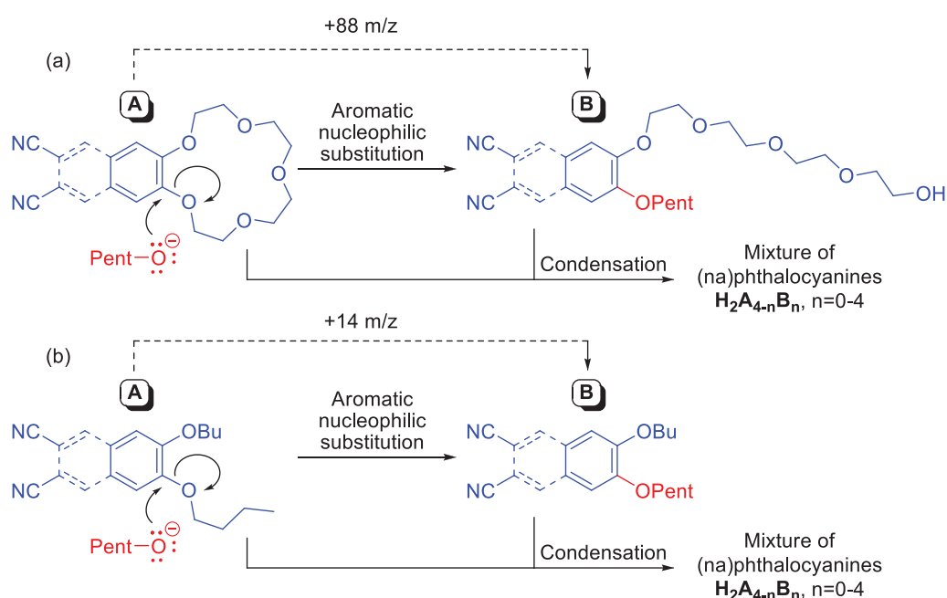
Figure 1. Products of \text{S}_{\text{N}}2_{\text{Ar}} reactions of crown-substituted dinitriles (a) and butoxy-substituted dinitriles (b) with pentoxide-anion.
