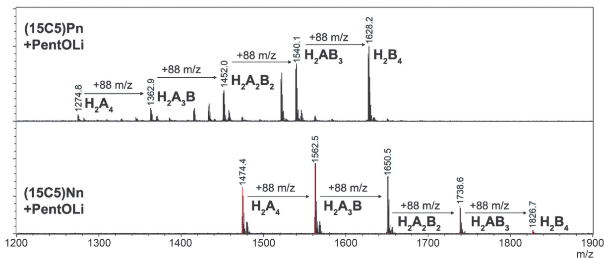
Figure 3. MALDI-TOF mass-spectra of reaction mixtures, formed upon cyclotetramerization of crown-substituted dinitriles in the presence of PentOLi in refluxing n -pentanol. “A” stands for intact isoindoline unit as a part of (na)phthalocyanine, “B” stands for the unit formed because of crown ether ring cleavage.
