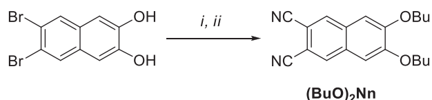
Scheme 1. Synthesis of (BuO) 2 Pn . i : n -BuBr, \text{K}_2\text{CO}_3 , DMF, 90 °C, Ar, yield – 75 %. ii : \text{Zn}(\text{CN})_2 , \text{Pd}_2(\text{dba})_3 , dppf, DMAA, 120 °C, Ar, yield – 95 %.
