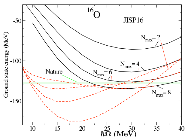
Fig. 1. Results for the ground state energy of ^{16}\text{O} with bare (solid) and LSO(2) renormalized (dashed) JISP16 interaction as a function of the oscillator parameter \hbar\Omega . When JISP16 was developed [20], the largest model space calculations where N_{\text{max}} = 6 .
