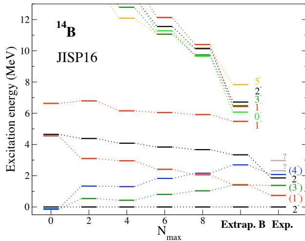
Fig. 3. Negative parity ^{14}\text{B} spectrum obtained with bare JISP16 interaction at fixed \hbar\Omega = 25 MeV in successive basis spaces, and extrapolated to infinite basis space using Extrapolation B. Experimental data are taken from Ref. [32].
