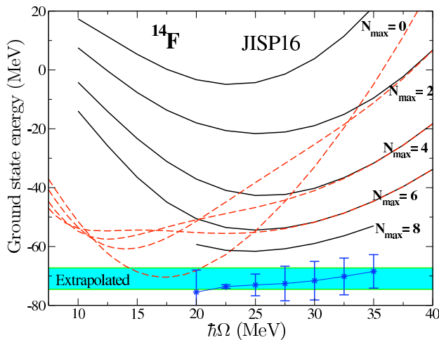
Fig. 2. Results for the ground state energy of ^{14}\text{F} with bare (solid) and effective (dashed) JISP16 interaction as a function of the oscillator parameter \hbar\Omega . The shaded area demonstrates the global extrapolation A for the binding energy and its uncertainty; the extrapolation B at fixed \hbar\Omega is given by stars with its uncertainties indicated by the error bars. The most reliable \hbar\Omega value for this extrapolation method is at \hbar\Omega = 25 MeV for ^{14}\text{F} .
