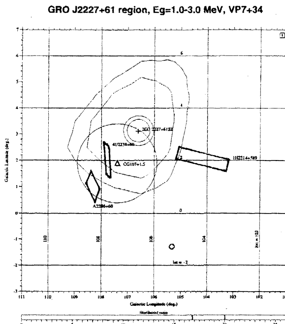
Fig. 1: Maximum-likelihood map of the GRO J2227+61 region for the combination of VP 7 and 34. The cross marks position of GRO J2227+61 (2EG 2227+6122). The triangle shows position of CG107+1.5. Contour lines are drawn at the 95 and 99% confidence level of the source position for COMPTEL and EGRET (stylized as a circle for EGRET). For the position of CG107+1.5 is given 90% confidence contour (Wills et al. 1979). The error boxes of the nearest X-ray sources are shown. Galactic coordinate grid is overlaid.
