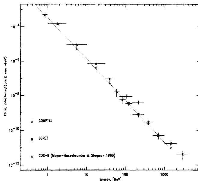
Fig. 2: The GRO J2227+61 spectrum include quasicon-temporaneous measurements by COMPTEL and EGRET, and non-contemporaneous COS-B measurement. The dotted line corresponds to the power law with a photon index of -2.20 \pm 0.14 , as derived from the EGRET measurements.
