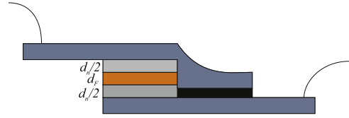
Figure 5. A schematic cross-section of the hybrid device with in-plane magnetization orientation and reduced inductive coupling. Ferromagnetic layer of thickness d_F (shown in orange) is placed between two nonmagnetic layers of total thickness d_n and in close proximity to the Josephson tunnel layer (shown in black).
