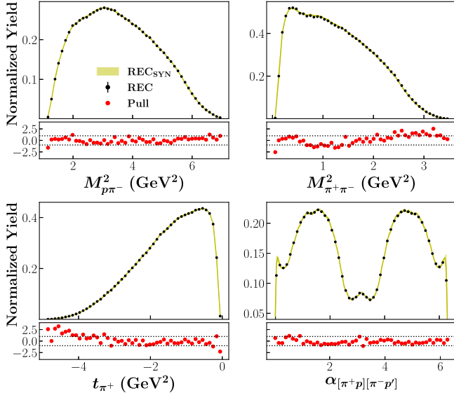
FIG. 11. Training variable PS-MC REC pseudodata distributions (black points) are compared to the synthetic data produced by the DS-GAN (yellow band). The band size reflects the uncertainty estimated using the bootstrap procedure, while the pull distributions (bottom of panels) quantify the agreement between the two, with the horizontal dotted lines corresponding to \pm 1\sigma .
