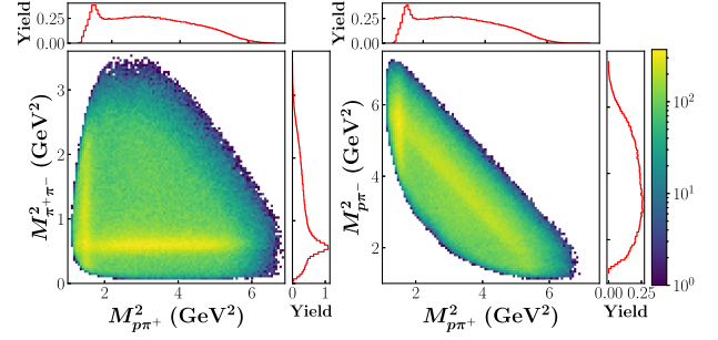
FIG. 1. Examples of 2D normalized yield distributions and their 1D projections measured in CLAS g11 experiment (before unfolding detector effects) [30]. Plots show invariant mass distributions for the yields M_{\pi^+ \pi^-}^2 versus M_{p\pi^+}^2 (left) and M_{p\pi^-}^2 versus M_{p\pi^+}^2 (right). For each 2D plot, the correspondent 1D projections are shown on top and right. The distributions are dominated by the prominent contributions from \Delta^{++} and \rho resonances, which appear as bands in the 2D distributions and peaks in the appropriate 1D projection. In particular, the \Delta^{++} appears as a vertical band in the 2D plots, and as a peak in the 1D M_{p\pi^+}^2 projection. The \rho is the horizontal band in the left 2D plot, the diagonal band in the right 2D plot, and the peak in the 1D M_{\pi^+ \pi^-}^2 yields. From the right plots one can see that, choosing M_{p\pi^+}^2 and M_{p\pi^-}^2 as independent variables, the existence of the \rho is lost if one studies the 1D projections only.
