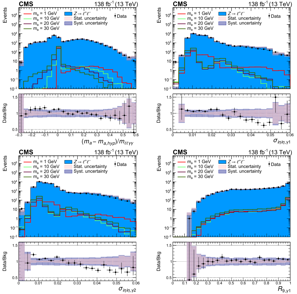
Fig. 2. Distributions of the four most discriminating variables used as input to the BDT: (m_a - m_{a,hyp})/m_{\ell\ell\gamma\gamma} (upper left), leading photon's \sigma_{in\eta, \gamma 1} (upper right), subleading photon's \sigma_{in\eta, \gamma 2} (lower left), and leading photon's R_9 (lower right). The events pass the selection criteria described in Section 5. The signal is scaled to a cross section of 0.1 pb and the background sample is normalized to an integrated luminosity of 138 \text{ fb}^{-1} . The systematic uncertainties included in the shaded band are related to the photon efficiency, lepton efficiency, and pileup modeling. The impact of the remaining disagreement between data and simulation is negligible.
