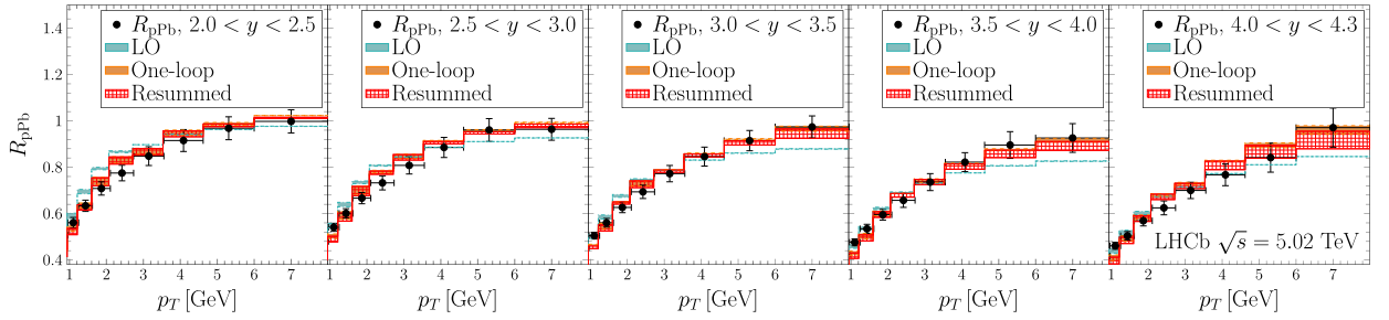
Fig. 28. LHCb Collaboration measurement of the nuclear modification factor of charge particles as a function of p_T in different rapidity intervals for the forward region in p + Pb collisions at \sqrt{s_{NN}} = 5 TeV at the LHC [673], compared to state of the art CGC calculations [674].
