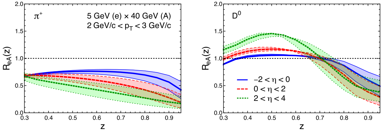
Fig. 51. Ratio of relative particle production ( N_h/N_{\text{incl}} ) in e+A over that in e+p as a function of z , the momentum fraction of the parton carried by the respective hadron. Light pions (left) show the largest nuclear suppression at the EIC. However, heavy flavor meson ratios (right) have to be measured to differentiate models of hadronization since they show a substantially different modification in e+A . (Figure is from [1380].)
