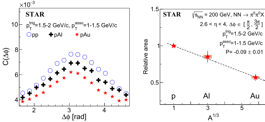
Fig. 29. Left: Comparison of correlations functions with azimuthal angle separation between forward ( 2.6 < \eta < 4.0 ) \pi^0 s in p + p , p + Al , and p + Au collisions at \sqrt{s_{NN}} = 200 GeV. Right: Relative area of back-to-back di- \pi^0 correlations in p + Au and p + Al with respect to p + p collisions for p_T^{trig} = 1.5-2 GeV/c and p_T^{asso} = 1-1.5 GeV/c.
