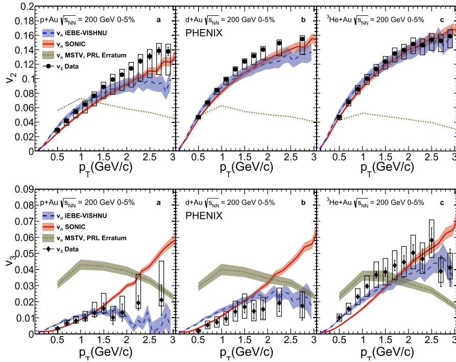
Fig. 11. Measurement of v_2 (top) and v_3 (bottom) for charged particles in p +Au, d +Au, and ^3\text{He} +Au collisions as a function of p_T . Calculations from two hydrodynamic models [354,355] and a CGC based model [356] are shown. Figure from Ref. [9].
