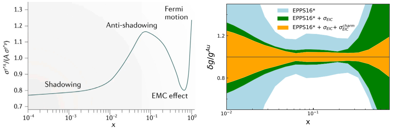
Fig. 50. Left: The cross section ratio \sigma^{rA}/(A\sigma^{rP}) measures the nuclear modification to the parton distribution functions (figure from [314]). Right: Relative uncertainty bands for the gluon distributions in gold nuclei at Q^2 = 1.69 GeV 2 . The blue band is the original EPPS16* fit, the green band incorporates inclusive cross section pseudodata and the orange band also adds the charm cross section \sigma^{charm} (figure from [1343]).
