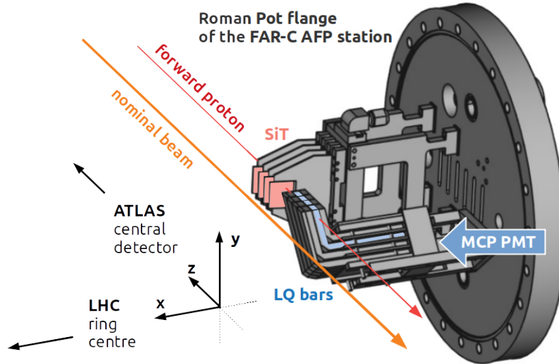
Figure 4. Schematic view of the AFP FAR-C station. For clarity, only the Roman pot flange without the cover is shown. The set of LQ-bars attached to the MCP-PMT is fixed in a holder which (together with the holder for the SiT) is mounted to the flange. The LQ bars traversed by the leading proton (shown as a red arrow) are highlighted in blue colour. Also the proton passage through the SiT tracker is indicated. The position of the nominal beam is shown by an orange arrow. The local right-handed reference frame is defined such that the positive x -axis is perpendicular to the flange and points to the LHC ring centre, the y -axis is perpendicular to the LHC ring plane and points upwards, and the positive z -axis represents the anticlockwise direction tangential to the LHC circumference pointing to the ATLAS IP.
