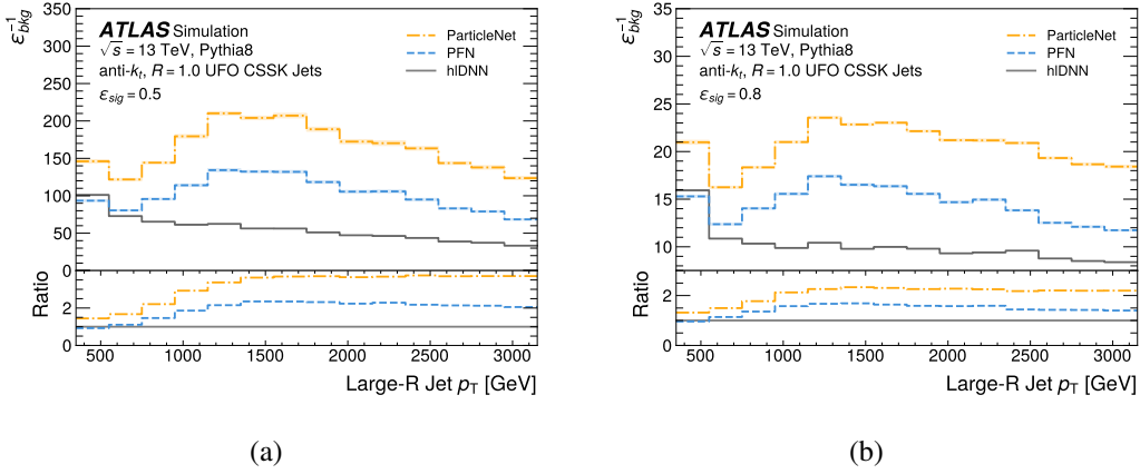
Figure 3. Background rejection, or inverse background efficiency ( \epsilon_{bkg}^{-1} ), of the hIDNN, PFN, and ParticleNet top quark taggers as a function of the jet p_T at the (a) 50% signal efficiency and (b) 80% signal efficiency working points. Shaded error bands are the quadrature sum of the error from the finite size of the testing set and the error from the random initialization of network weights and the stochastic nature of network training.
