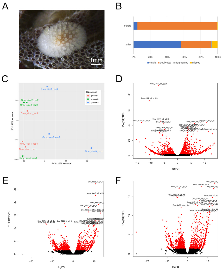
Fig. 1. Transcriptome completeness and differential expression in Onchidoris muricata . (A) O. muricata in natural environment. (B) BUSCO scores before and after decontamination of assembly. (C) Expression levels in three size groups were analyzed using the principal component analysis (PCA) method. The 500 genes with most variable expression were analyzed. (D) Differential transcript expression in groups I and II. Each dot on the graph represents a transcript; black dots have p-value > 0.05, red dots have p-value < 0.05. Red dots to the right of zero on the abscissa axis are transcripts with log fold change (L2FC) greater than one in group I (i.e., up-regulated in this group), and to the left of zero are transcripts with L2FC > 1 in group II. On the abscissa axis is L2FC, on the ordinate axis is the decimal logarithm of p-value. (E) Differential transcript expression in groups I and III. (F) Differential transcript expression in groups II and III.
