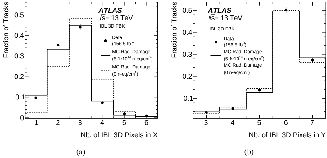
Figure 9. Number of pixels in the (a) transverse (local X) and (b) longitudinal (local Y) projection for IBL 3D sensors with clusters associated with reconstructed particle tracks. Points with error bars represent data in 13 TeV collision events collected in 2018 after 156.5 \text{ fb}^{-1} of integrated luminosity and are compared with the predictions of ATLAS radiation damage simulation for fluences of 0 (dashed line) and 5.1 \times 10^{14} \text{ n-eq cm}^{-2} (continuous line). The larger pixel multiplicity in the longitudinal projection is dominated by the affect of the shallow angle of incidence of particle tracks in the IBL module region equipped with 3D sensors.
