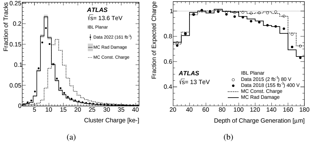
Figure 4. (a) Distribution of cluster charges in IBL planar sensors from data taken in 2022, after an estimated average fluence of about 8.7 \times 10^{14} \text{ n-eq cm}^{-2} , at a bias voltage of 450 V (points with error bars). The predictions from simulated events with (without) radiation damage effects are shown by the continuous (dashed) histograms. (b) Charge collection efficiency as a function of the estimated depth of charge generation for IBL planar sensors in 13 TeV collision data, at the start of Run 2 in 2015 ( 2 \text{ fb}^{-1} of integrated luminosity) shown by the open points and at the end of Run 2 in 2018 ( 156 \text{ fb}^{-1} of integrated luminosity) shown by the filled points, and radiation damage simulation for matching fluence conditions. The efficiency is computed by comparing the fraction of the cluster charge deposited on the pixels ordered from the extrapolated point of track entrance in the Si substrate to that of track exit in the longitudinal projection. The drops observed at the two ends of the depth range are due to resolution effects. To optimise the resolution, only tracks with p_T > 3 \text{ GeV} and at least three pixels in the longitudinal projection are considered.
