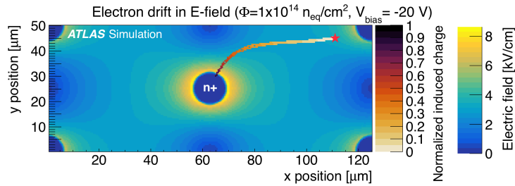
Figure 6. Electric field and normalised induced charge in one-half of a 3D sensor for a simulated bias voltage of -20 \text{ V} . The initial electrons are ionised in the top right corner of the plot, indicated by a star. Under the influence of the electric field, they drift toward the n^+ electrode in the centre. During this drift, the electrons may get trapped. The markers indicate the location of trapped charges and the marker colour shows the corresponding fraction of the deposited charge induced on the read-out electrode. The process is repeated multiple times, accounting for diffusion effects. Reproduced from [7]. © 2019 CERN for the benefit of the ATLAS collaboration. CC BY 3.0.
