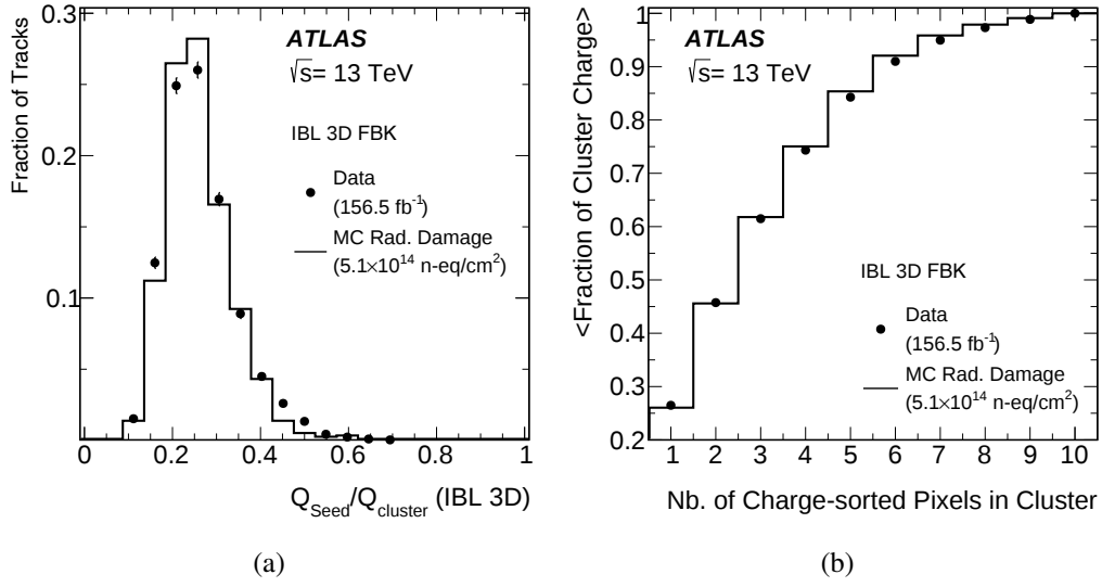
Figure 10. Charge sharing in 3D clusters for 3D FBK sensors in 13 TeV collision events collected after 156 fb -1 of integrated luminosity: (a) fraction of the total cluster charge carried by the pixel with the highest charge (“seed pixel”) and (b) average cumulative fraction of the cluster charge as a function of the number of contributing pixels, sorted in order of decreasing pixel charge. Points represent data and the histogram shows the radiation damage simulation.
