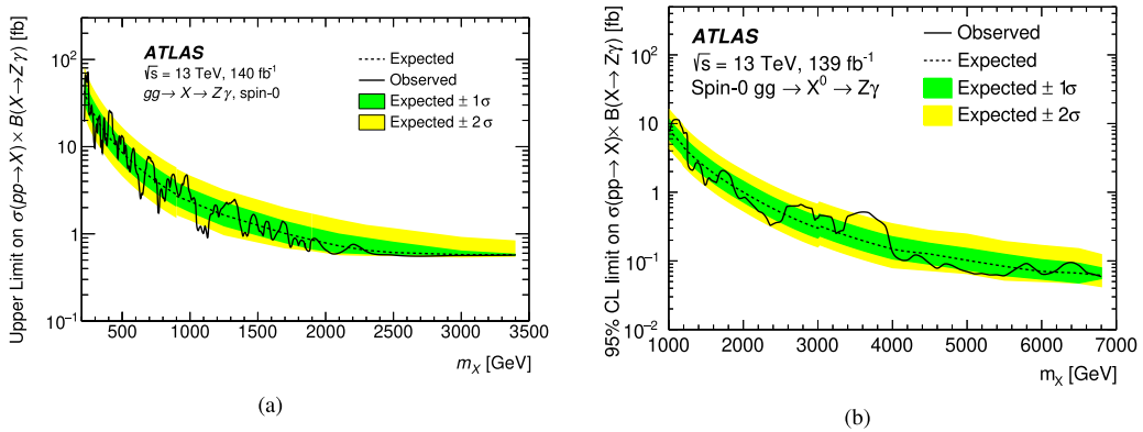
Fig. 22. X \rightarrow Z\gamma : The 95% CL limit on the cross-section times branching fraction as a function of the mass of the narrow-width scalar X in the case where the Z boson decays (a) into either electrons or muons, or (b) via the hadronic decay mode. The limits in (b) have a small discontinuity at 3 TeV because the category exploiting b -tagging is dropped for higher masses.
