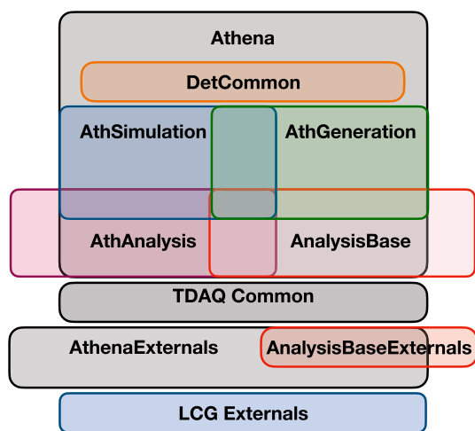
Fig. 26 Schematic overview of the ATLAS software projects and external dependencies. The overlaps between project areas indicate overlaps in code included in the projects. The widths of AnalysisBase-Externals and AthenaExternals are wider to indicate their support for the entirety of the AnalysisBase and AthAnalysis projects, respectively
